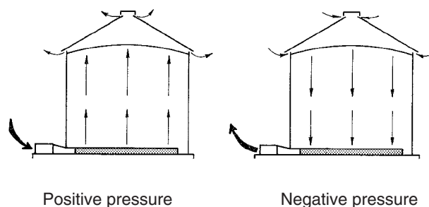
Figure 2. Grain bin airflow directions.
